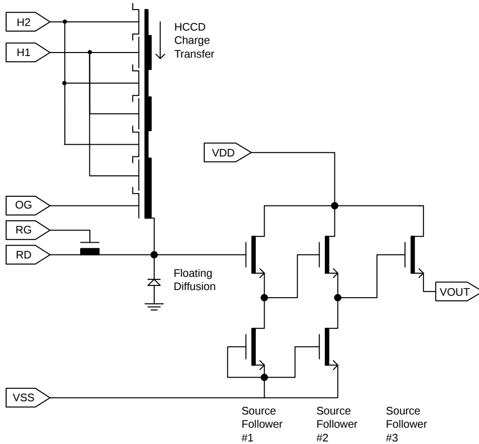
Figure 3. Output Architecture
