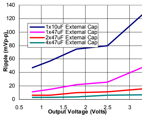
Figure 29. Output ripple voltage for various output voltages with external 1x10 µF, 1x47 µF, 2x47 µF or 4x47 µF ceramic capacitors at the output (30A load). Input voltage is 12V.
