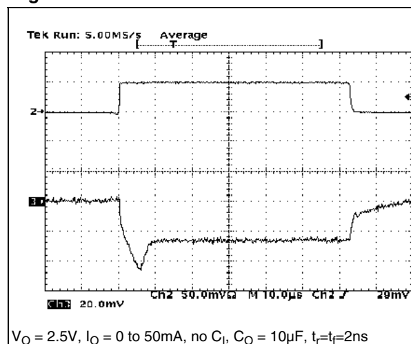
Figure 15. Load transient
