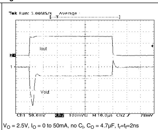
Figure 16. Load transient
