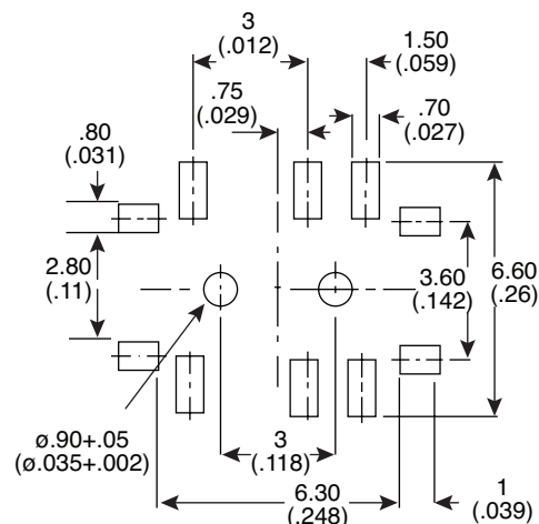
PCB Layout
