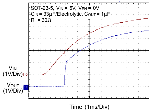
UVLO at Rising
