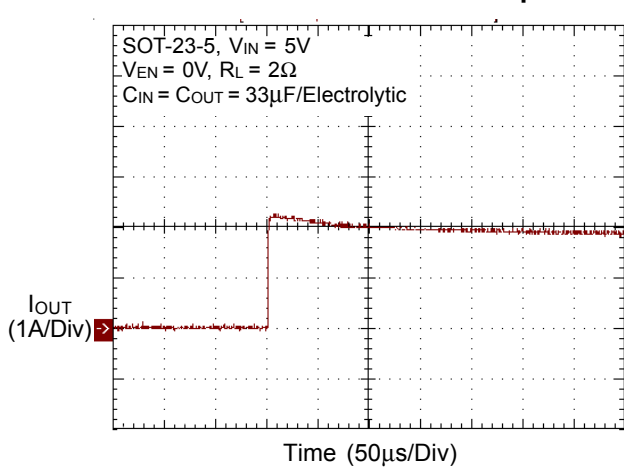
Current Limit Transient Response
