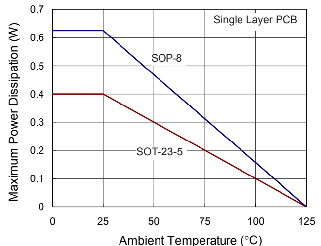
Figure 1. Derating Curves for RT9711 Package
