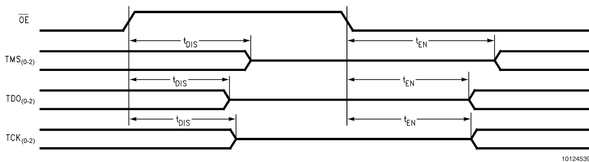
FIGURE 17. Output Enable Waveforms
