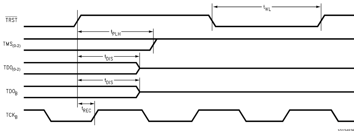
FIGURE 16. Reset Waveforms
