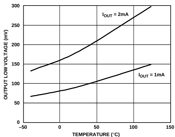
Figure 12. Output Low Voltage vs. Temperature
