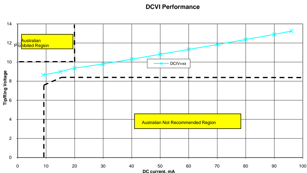
Figure 33: Voltage versus Current in the Seize Mode is the Same for All DCIV Settings
