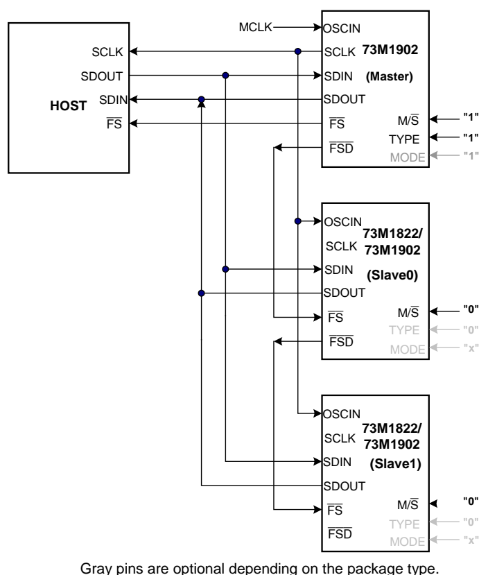
Figure 23: Daisy Chaining a Master and Two Slaves
