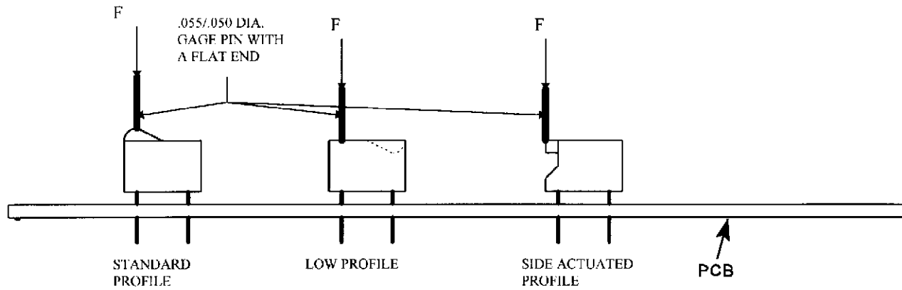
Figure 4 Actuation Force
