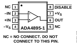
Figure 1. ADA4895-1 Single Amplifier (8-Lead SOIC)
