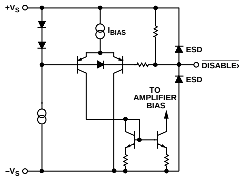
Figure 45. DISABLEx Circuit
