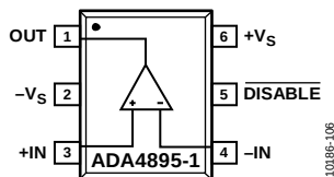
Figure 6. 6-Lead SOT-23 Pin Configuration for the ADA4895-1
