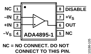
Figure 5. 8-Lead SOIC Pin Configuration for the ADA4895-1
