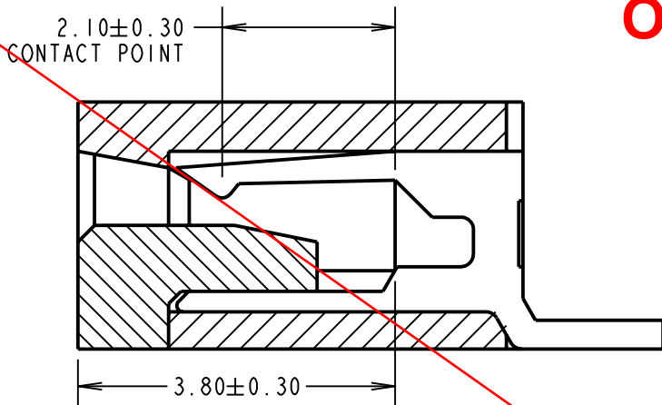
SECTION X-X ACTUATOR CLOSED
