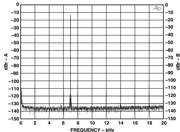
Figure 20. Two-Tone Test
