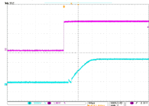
Start-up I_o=2A , V_o=1.2V , V_{in}=3.3V
