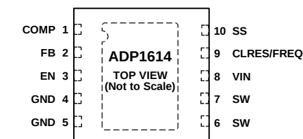
Figure 3. Pin Configuration
