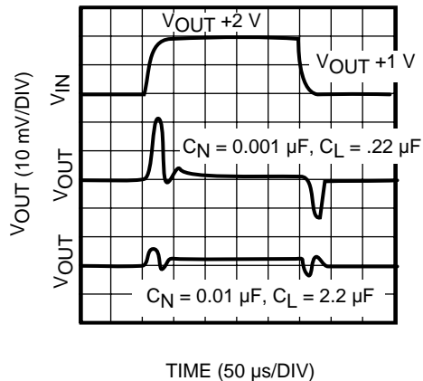
LINE VOLTAGE STEP RESPONSE
