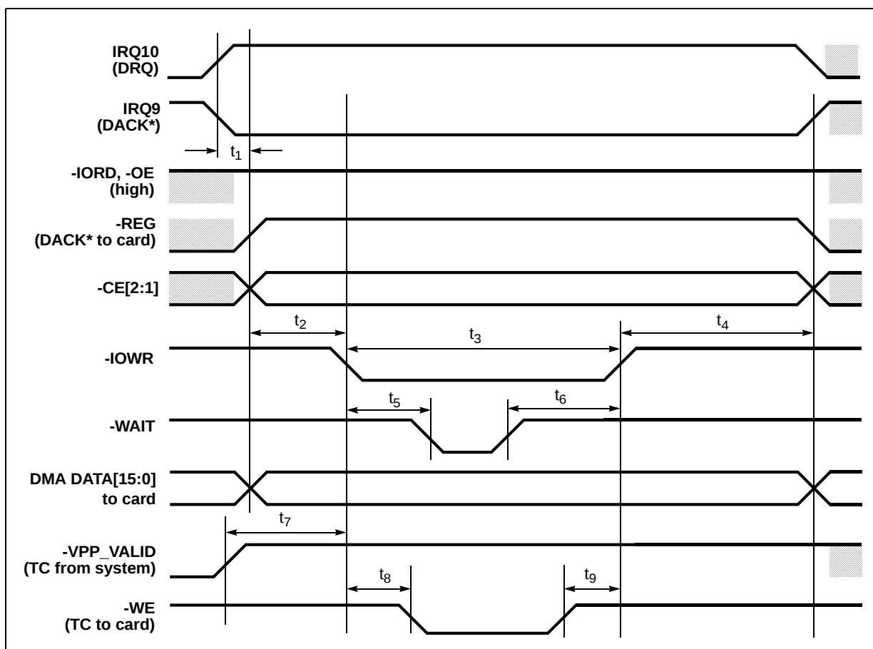
Figure 28. DMA Read Cycle Timing
