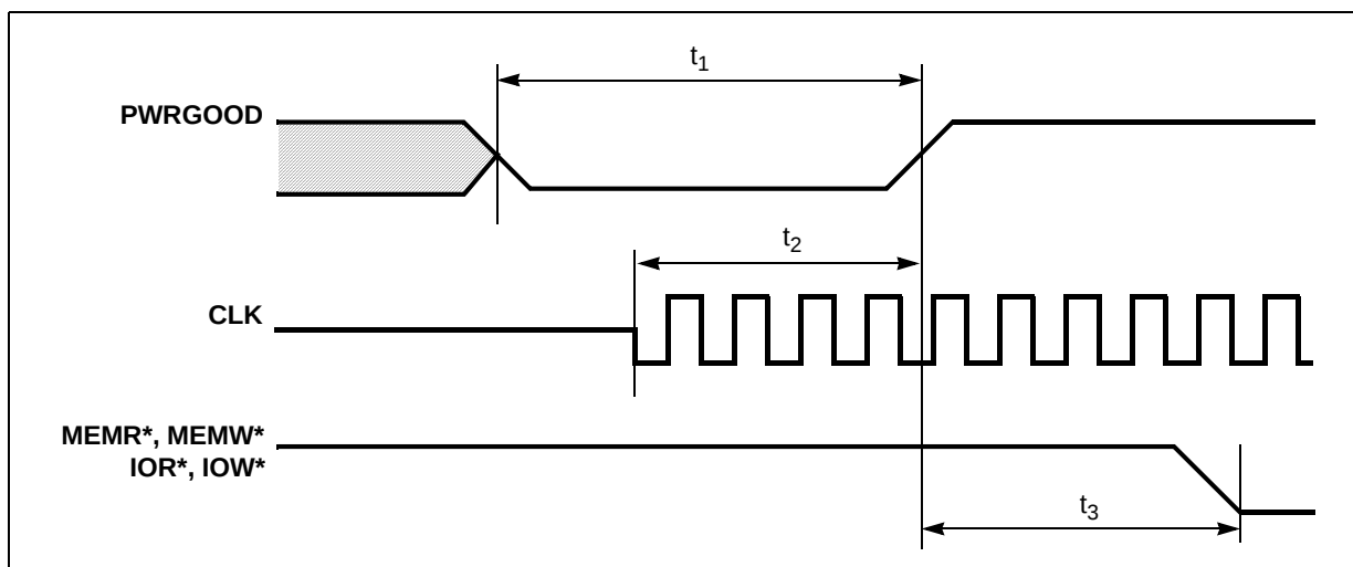
Figure 19. Reset Timing
