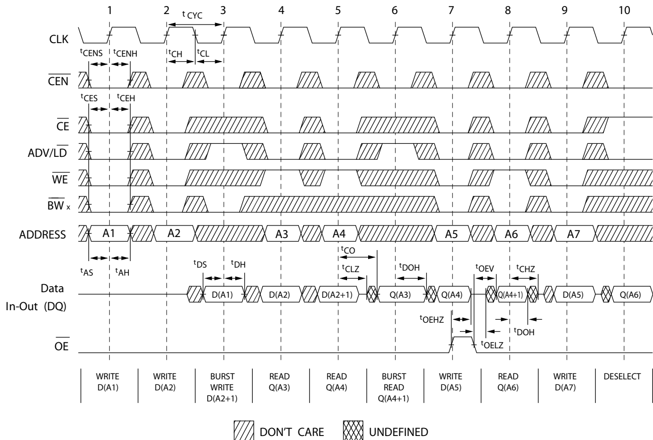
Figure 5. Read/Write Timing
