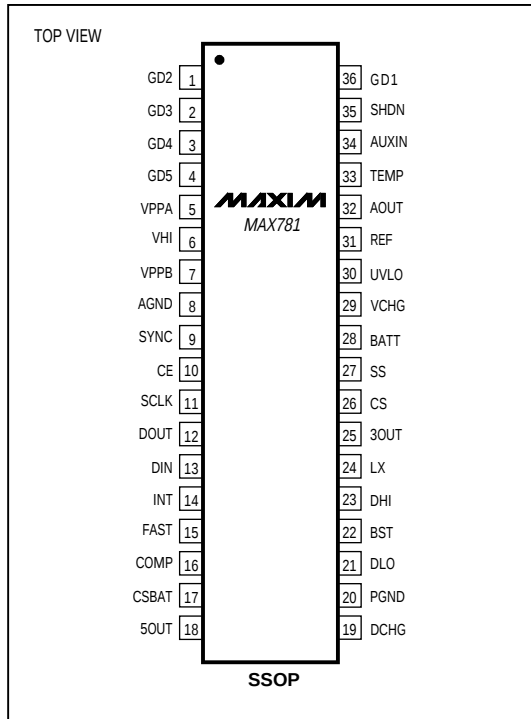
Pin Configuration
