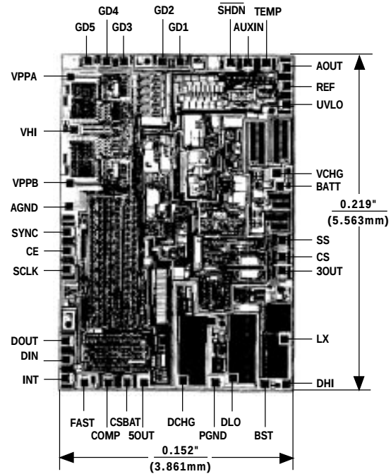
Chip Topography
