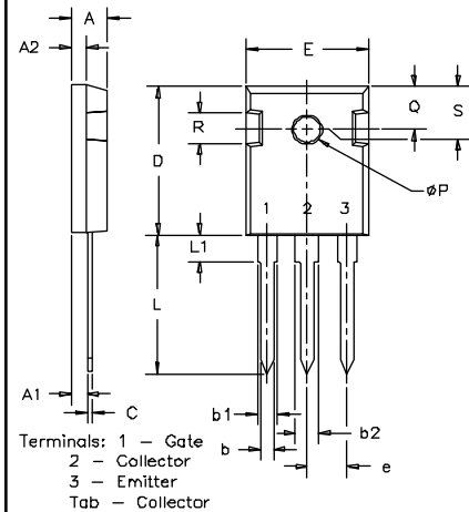
TO-247AD (IXSH)
