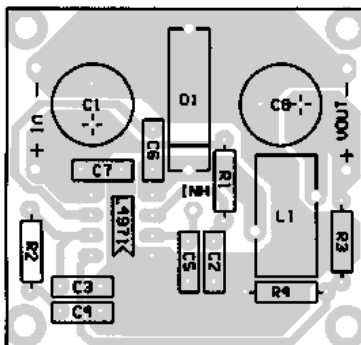
Figure 5. PCB and component layout of the figure 4.
