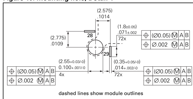
Figure 10. Mounting hole, Detail Y
