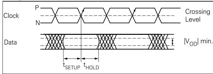
Figure 6. Measurement conventions for LVDS signals
