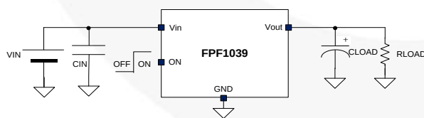
Figure 33. Device Setup
