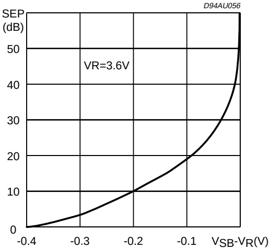
Figure 2: Stereo Blend
