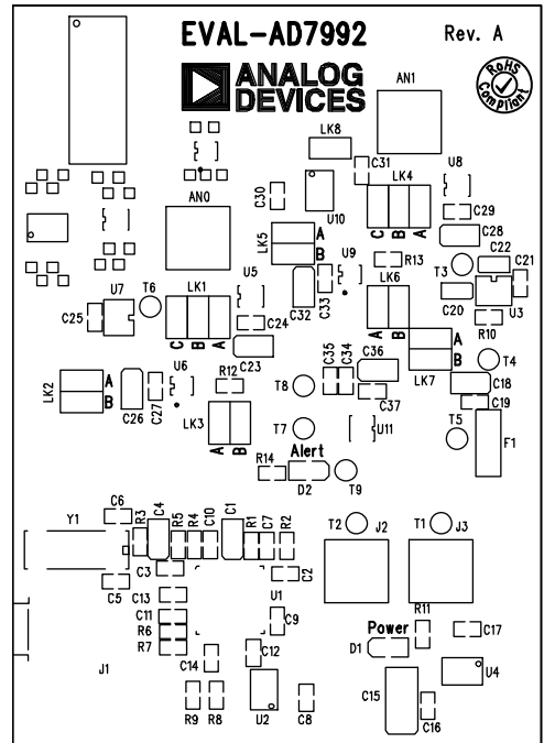
Figure 7. Component Placement Drawing
