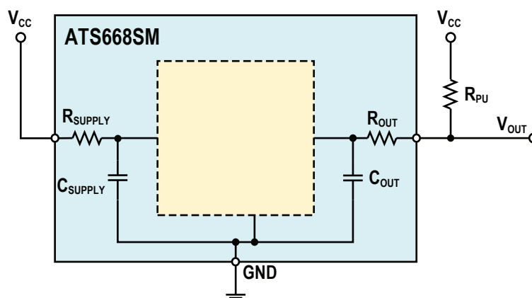
Figure 1: Typical Application
