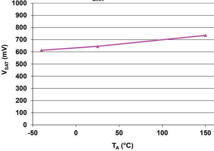
Output Voltage versus Ambient Temperature I_{SINK} = 10\text{ mA}
