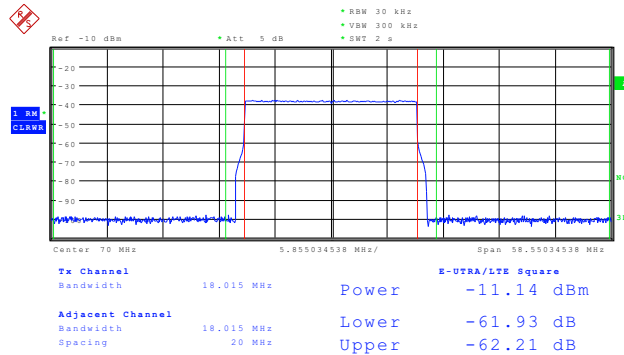
Figure 22. DAC3154 ACPR LTE 20-MHz FDD E-TM 1.1
