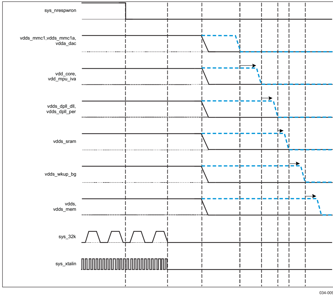
Figure 3-4. Power-down Sequence
