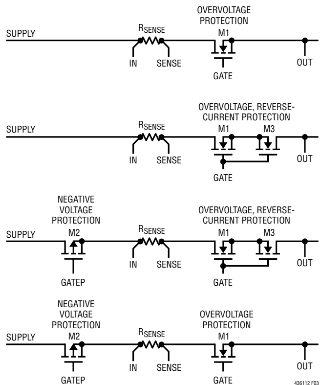
Figure 3. MOSFET Configurations
