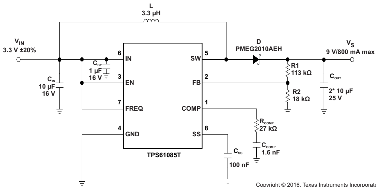
Figure 15. Typical Application, 3.3 V to 9 V ( f_{sw} = 1.2 MHz)
