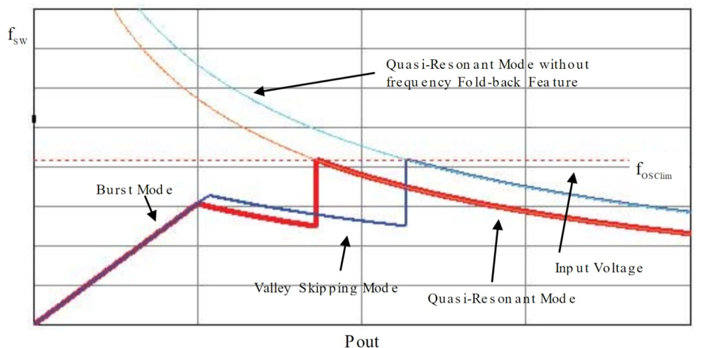
Figure 32. Switching frequency vs power
