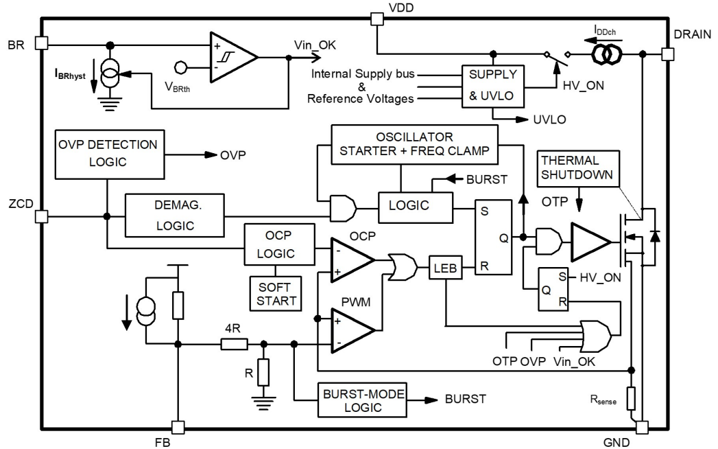
Figure 1. Block diagram
