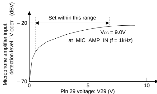
Fig. 7 Microphone amplifier input detection level vs. pin 29 voltage
