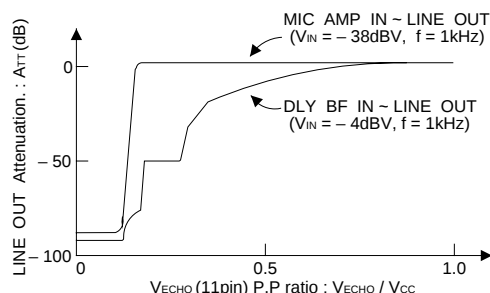
Fig. 2 LINE OUT attenuation ratio vs. V echo (11pin) partial pressure ratio
