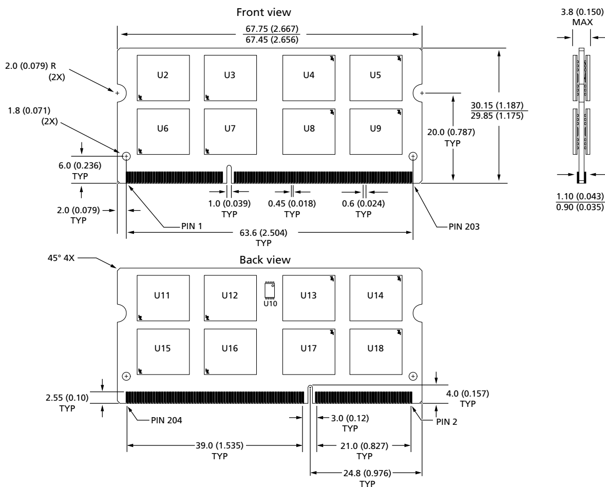
Figure 5: 204-Pin DDR3 SODIMM (PCB 1569, R/C-F3)
