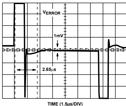
FIGURE 10. SETTLING WAVEFORM
