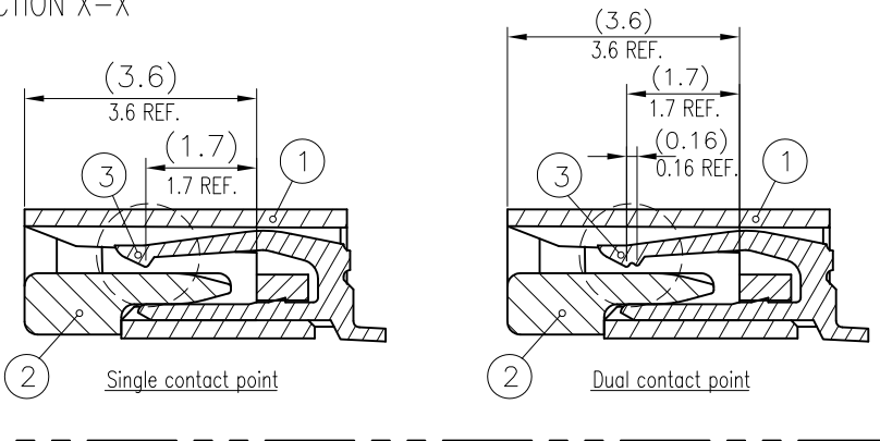
SECTION X-X
