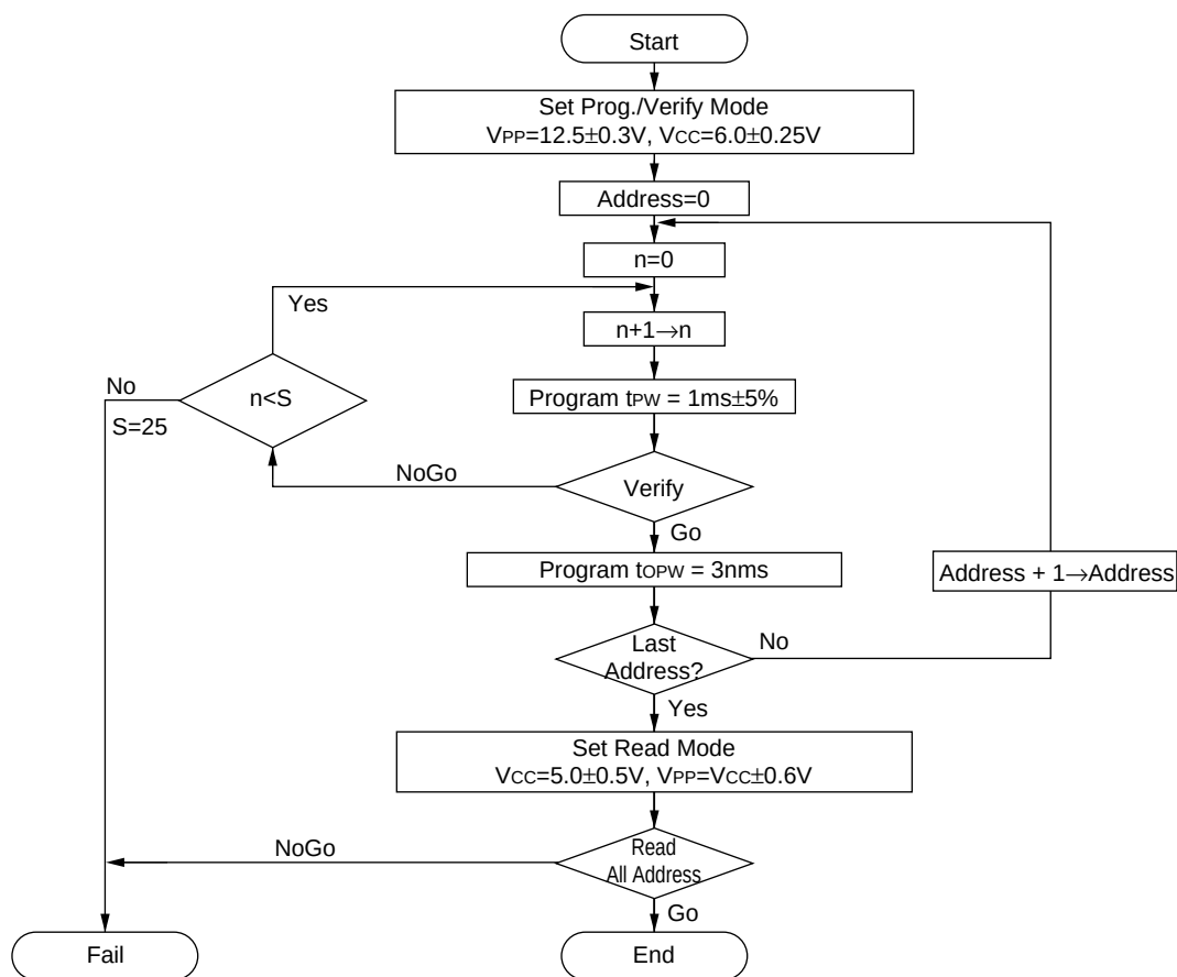
Figure 71 Flowchart of High-Speed Programming
