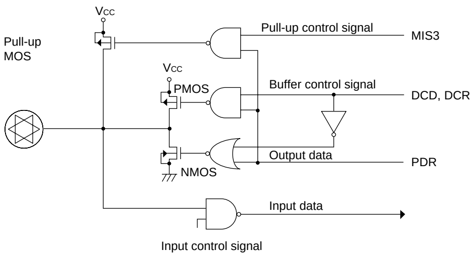
Figure 24 I/O Pin Circuit Configuration
