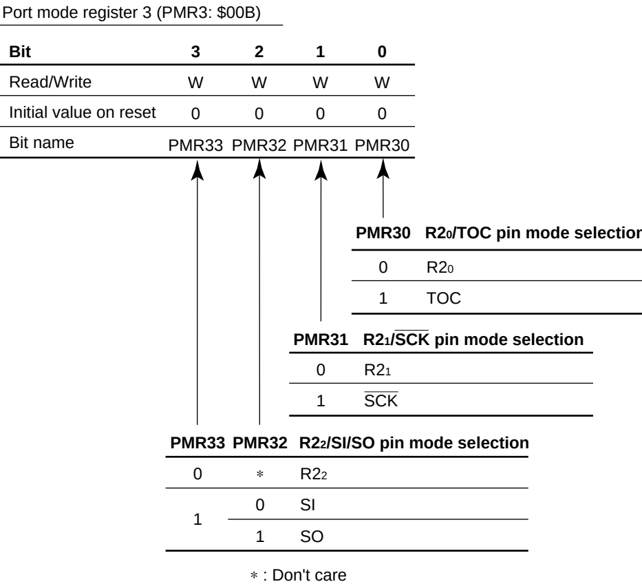
Figure 61 Port Mode Register 3 (PMR3)
