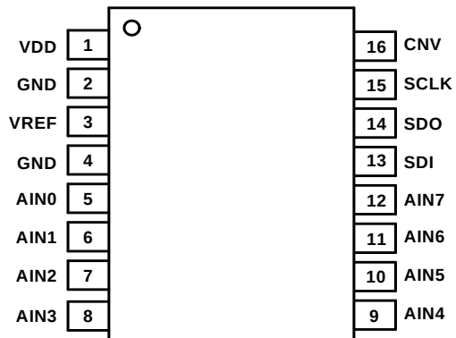
ISL26329 (16 LD TSSOP) TOP VIEW
