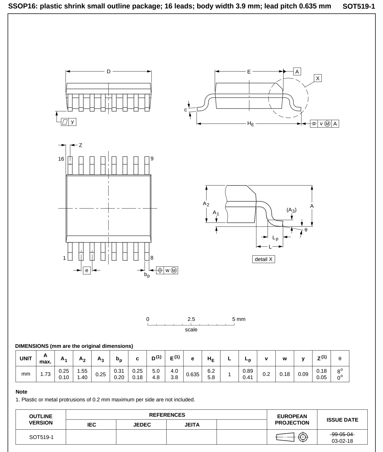
Fig 14. Package outline SOT519-1 (SSOP16)
