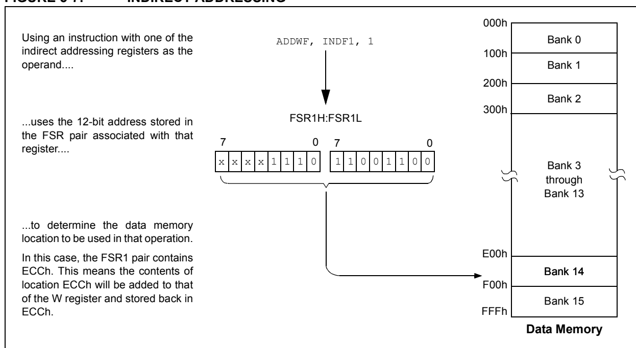
FIGURE 5-7: INDIRECT ADDRESSING
