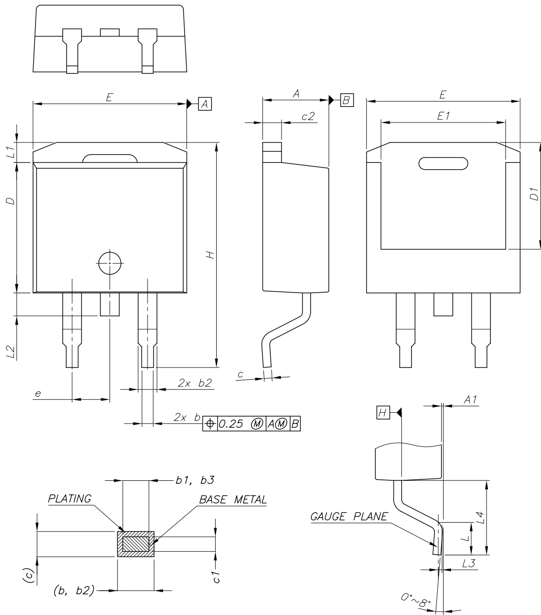
Figure 45. D 2 PAK (ASE subcon) type B package outline
