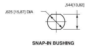
SNAP-IN BUSHING
