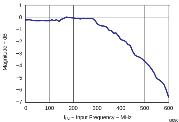
Figure 93. ADC Analog Input Bandwidth
