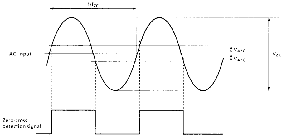
Figure 2-8. Zero-cross detection signal
