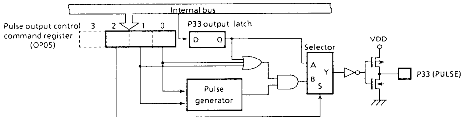
Figure 2-3. Pulse generator
