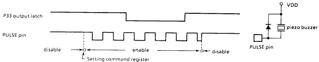
Figure 2-5. Timing chart and circuit example of buzzer pulse
