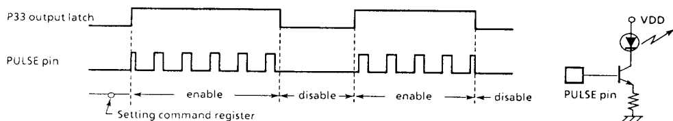
Figure 2-6. Timing chart and circuit example of carrier pulse for Remo-con
