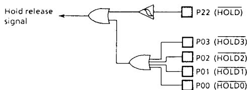
Figure 3-1. Hold control circuit
