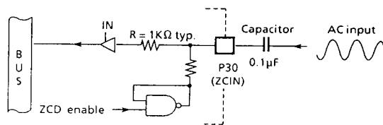
Figure 2-7. Zero-cross detector
