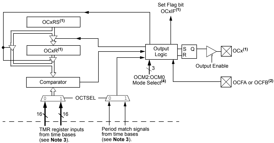
FIGURE 13-1: OUTPUT COMPARE MODULE BLOCK DIAGRAM
