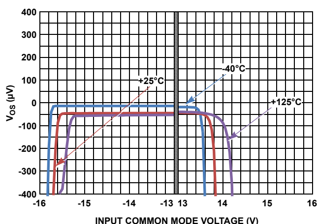
FIGURE 2. INPUT OFFSET VOLTAGE vs INPUT COMMON MODE VOLTAGE, V_{\text{S}} = \pm 15\text{V}
