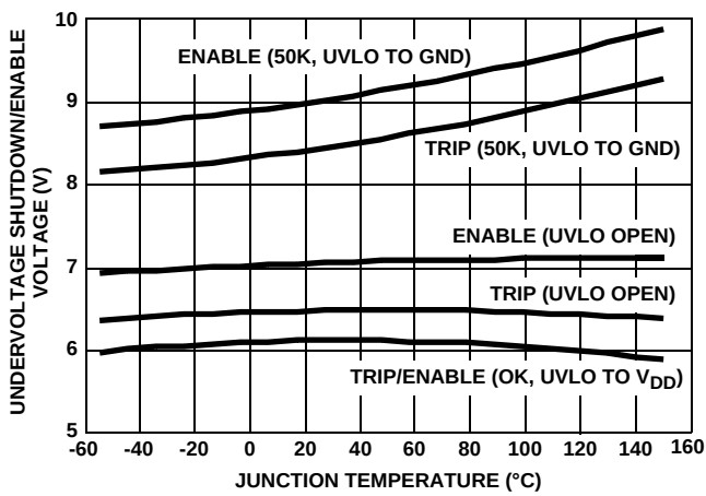
FIGURE 7. UNDERVOLTAGE THRESHOLD
