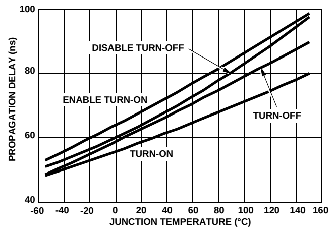
FIGURE 8. PROPAGATION DELAY
