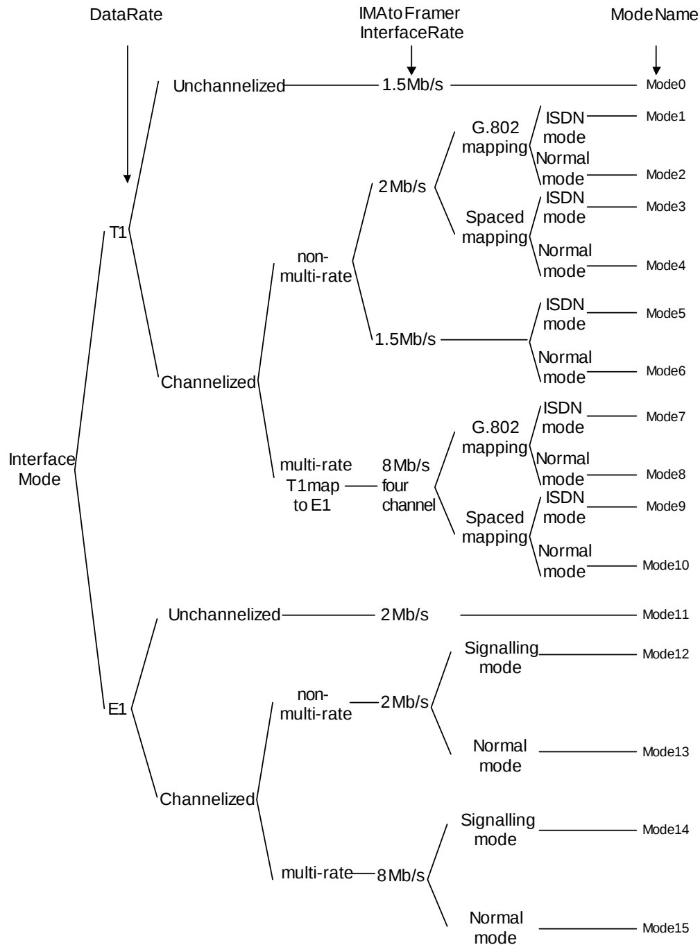
Figure-4 Line Interface Work Modes
