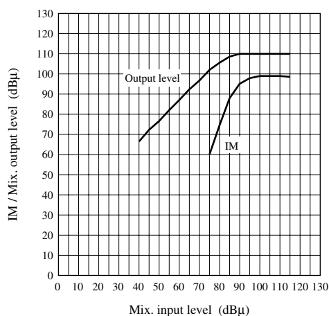
AN6591FJM Mix. characteristics
