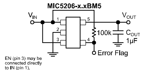
Figure 1a. Low-Noise Fixed Voltage Application
