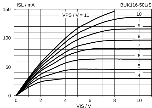
Fig.24. Typical latched input characteristics, 25 \text{ °C} . I_{ISL} = f(V_{IS}) ; after overload protection latched
