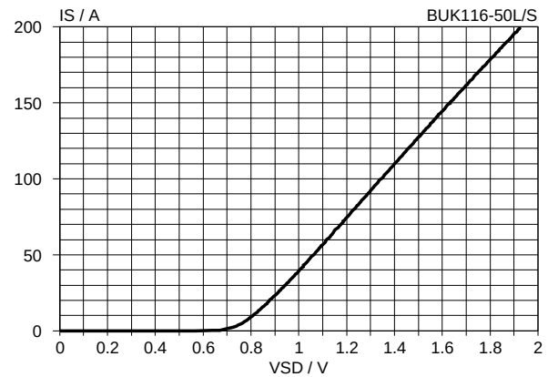
Fig.25. Typical reverse diode current, T_J = 25 \text{ °C} . I_S = f(V_{DS}) ; conditions: V_{IS} = 0 \text{ V} ; t_p = 250 \text{ μs}
