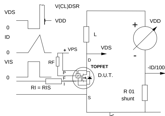
Fig.27. Clamping energy test circuit, R_{IS} = 100 \text{ Ω} . E_{DSM} = 0.5 \cdot L I_D^2 \cdot V_{(CL)DSR} / (V_{(CL)DSR} - V_{DD})
