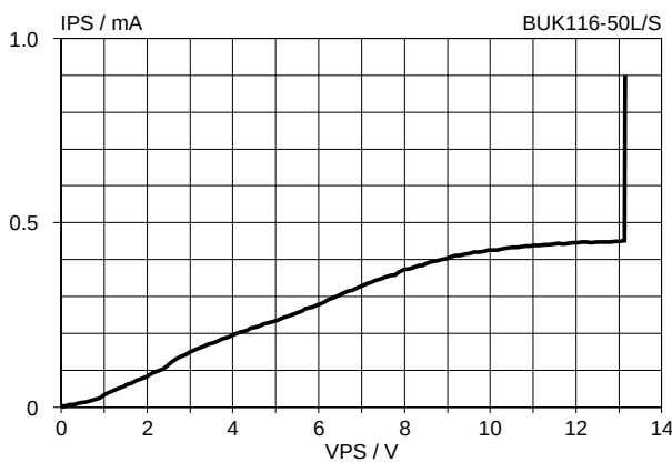
Fig.23. Typical DC protection supply characteristics. I_{PS} = f(V_{PS}) ; normal or overload operation; T_J = 25 \text{ °C}
