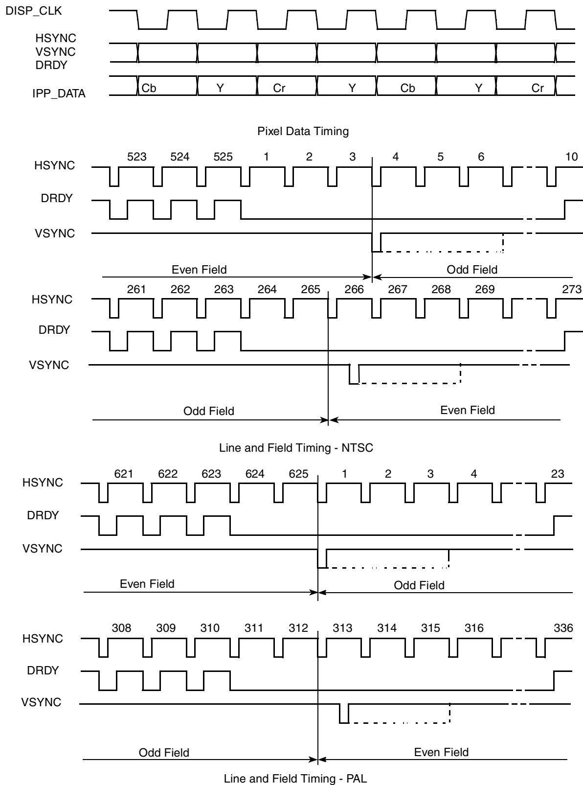
Figure 57. TV Encoder Interface Timing Diagram
