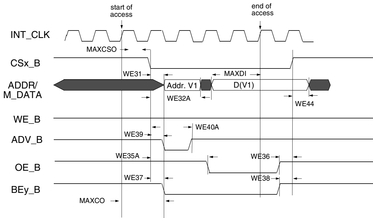
Figure 27. Asynchronous A/D Muxed Read Access (RWSC = 5)
